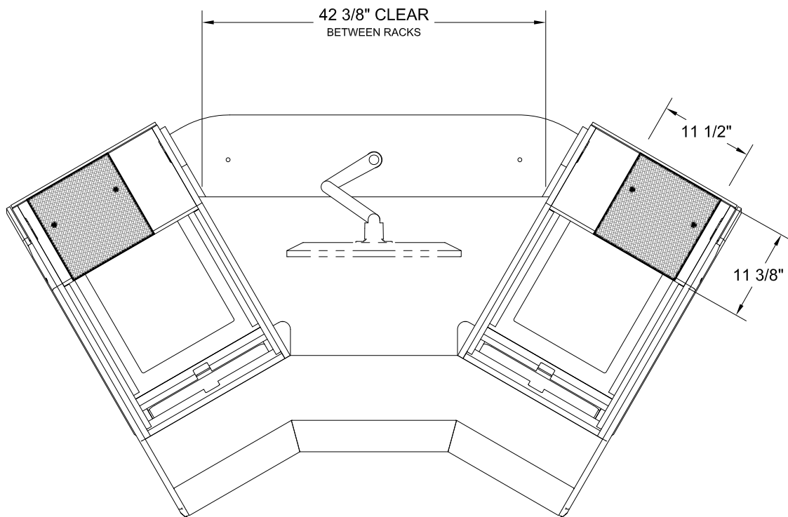
PLAN VIEW
