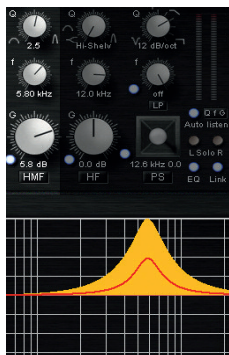
Auto listen "Q" with positive gain [see the HMF band gain at (+5.8dB)]
