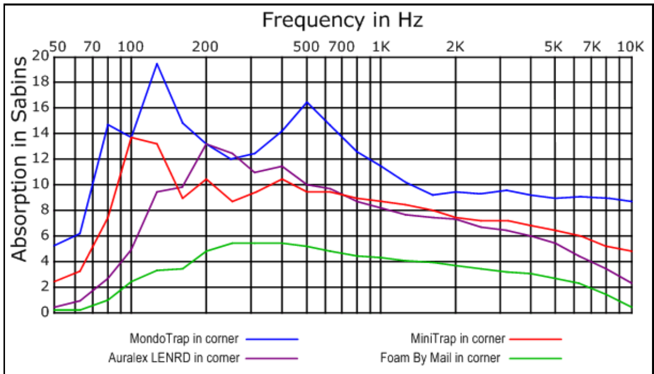
Absorption Comparison - values are Sabins per 4-foot unit (MondoTraps are 4'-9")
