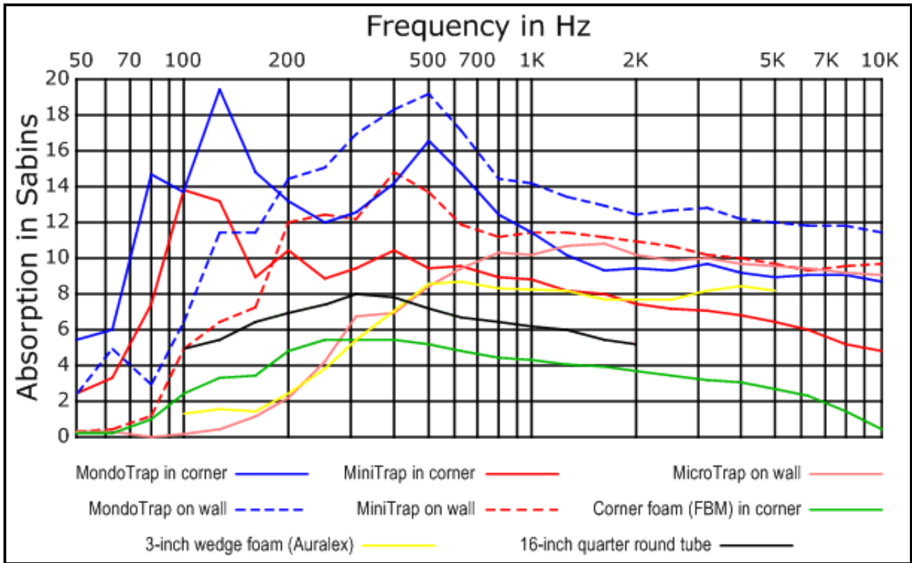
Absorption Comparison - values are Sabins per 4-foot unit (MondoTraps are 4'-9") (Some products are omitted to avoid clutter, complete data is in the tables below.)
